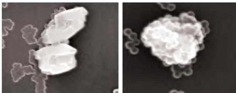
Figure 2: Left picture shows a SEM micrograph (50K magnification) of calcium carbonate dispersed in a Conventional acrylic latex polymer. Picture on right shows calcium carbonate dispersed in AVANSE™ MV-100 Resin. The latex particles appear as the smaller, grey spheres, and calcium carbonate appears as white.
